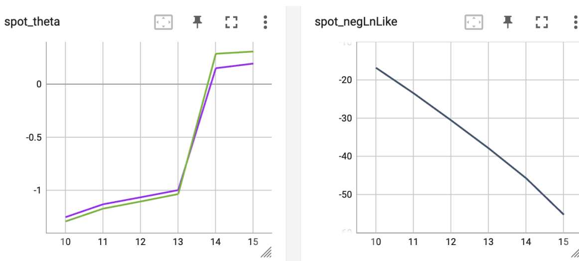
Figure 9.1: TensorBoard visualization of the spotPython surrogate model.
