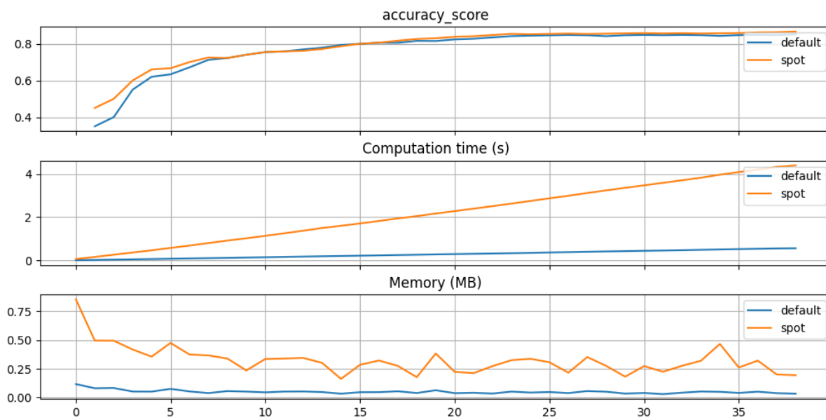
Figure 19.14: Default versus tuned hyperparameters
