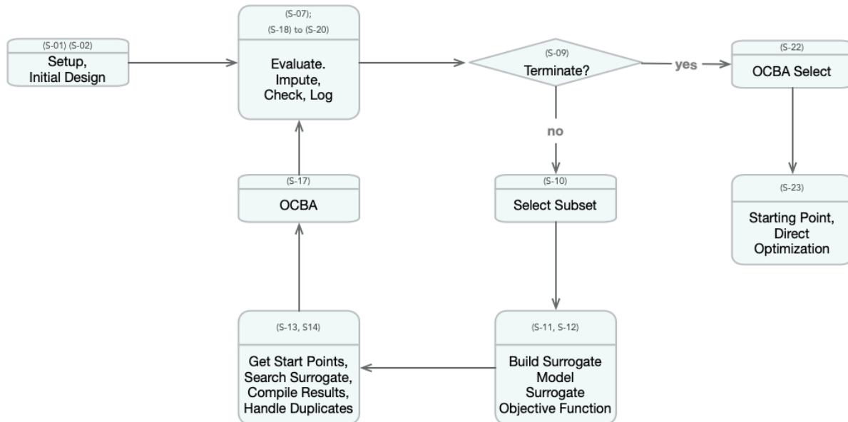
Figure 12.4: Visual representation of the model based search with SPOT. Taken from: Bartz-Beielstein, T., and Zaefferer, M. Hyperparameter tuning approaches. In Hyperparameter Tuning for Machine and Deep Learning with R - A Practical Guide, E. Bartz, T. Bartz-Beielstein, M. Zaefferer, and O. Mersmann, Eds. Springer, 2022, ch. 4, pp. 67–114.
