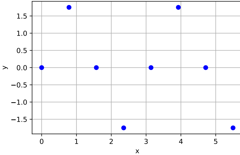
Figure 6.10: Eight measurements of an unknown function
