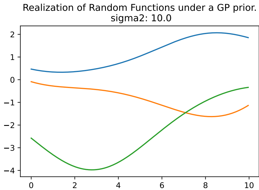
Figure 6.8: Realization of Random Functions under a GP prior. sigma2: 10
