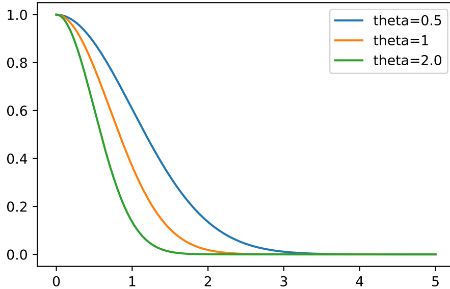
Figure 6.11: Theta set to 1/2, 1, and 2
