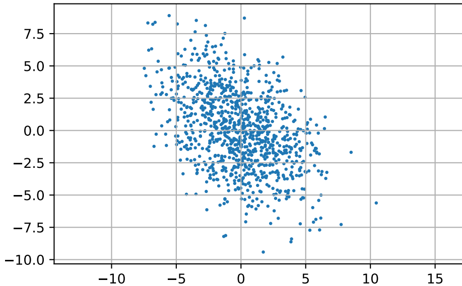
Bivariate Normal. Mean zero and covariance: [[9, -4], [-4, 9]]
