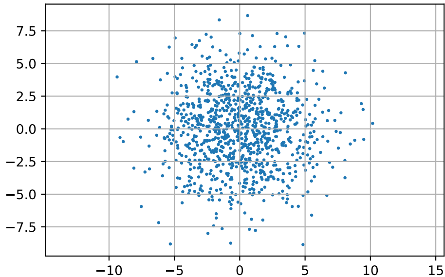
Figure 6.3: Bivariate Normal. Mean zero and covariance \Sigma = \begin{pmatrix} 9 & 0 \\ 0 & 9 \end{pmatrix}
