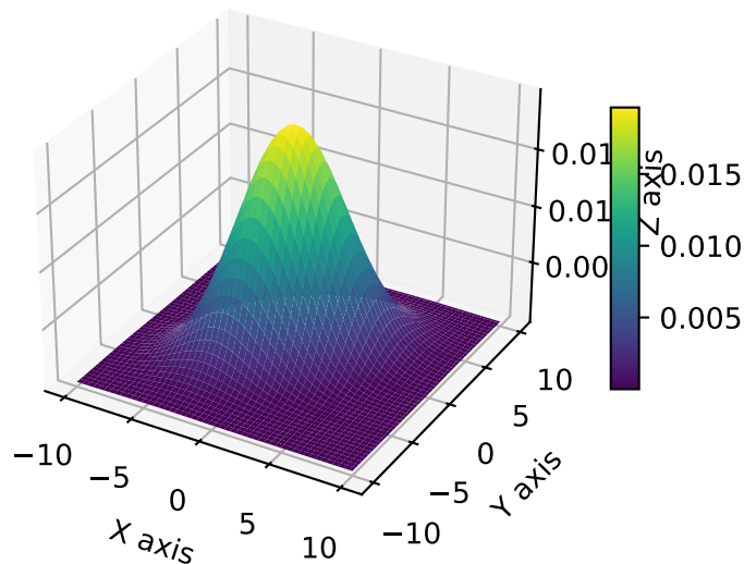
Figure 6.2: Bivariate Normal. Mean zero and covariance \Sigma = \begin{pmatrix} 9 & 4 \\ 4 & 9 \end{pmatrix}
