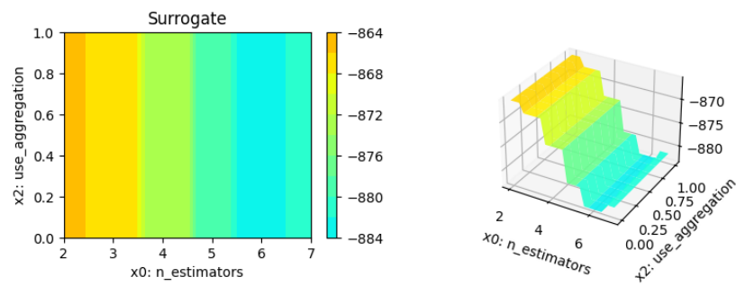
Figure 19.17: Surrogate plot based on the Kriging model. x_0 and x_2 plotted against each other.
