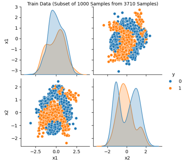
Figure 19.5: Visualization of the train data. Output from the spotRiverGUI when Bananas data is selected for the Show Data option
