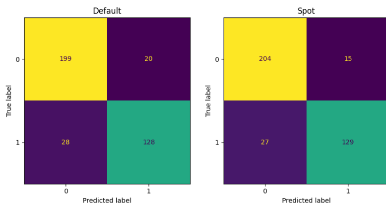
Figure 19.13: Confusion matrix
