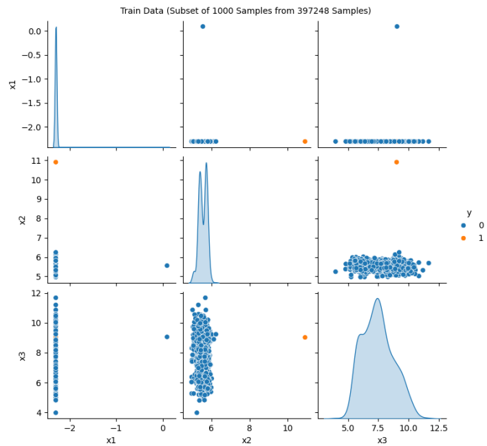
Figure 19.8: Output from the spotRiverGUI when HTTP data is selected for the Show Data option. A subset of 1000 randomly chosen data points is shown. Only a few positive events are in the data.
