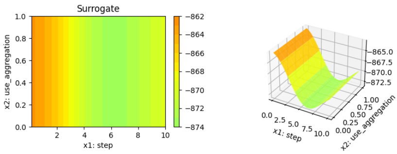
Figure 19.16: Surrogate plot based on the Kriging model. x_1 and x_2 plotted against each other.
