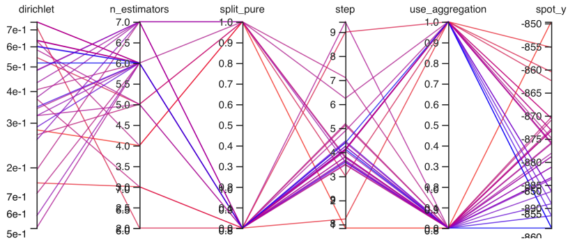
Figure 19.11: Tensorboard. Parallel coordinates plot
