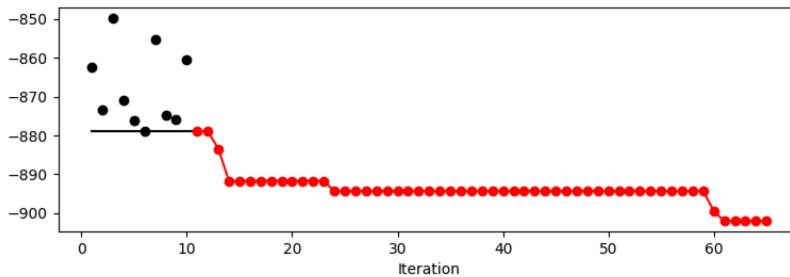
Figure 19.12: Progress plot of the hyperparameter tuning process
