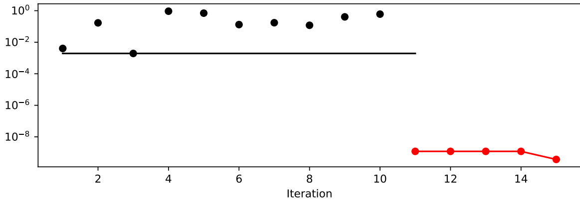
Figure 7.1: Visualization of the search progress of the Spot method. The black elements (points and line) represent the initial design, before the surrogate is build. The red elements represent the search on the surrogate.
