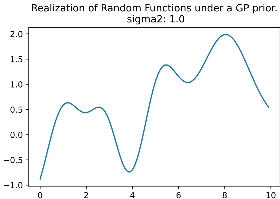
Figure 6.6: Realization of one random function under a GP prior. sigma2: 1.0
