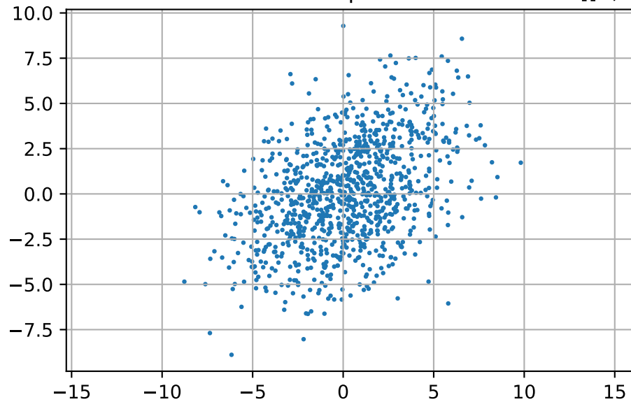
Figure 6.1: Bivariate Normal. Mean zero and covariance \Sigma = \begin{pmatrix} 9 & 4 \\ 4 & 9 \end{pmatrix}
