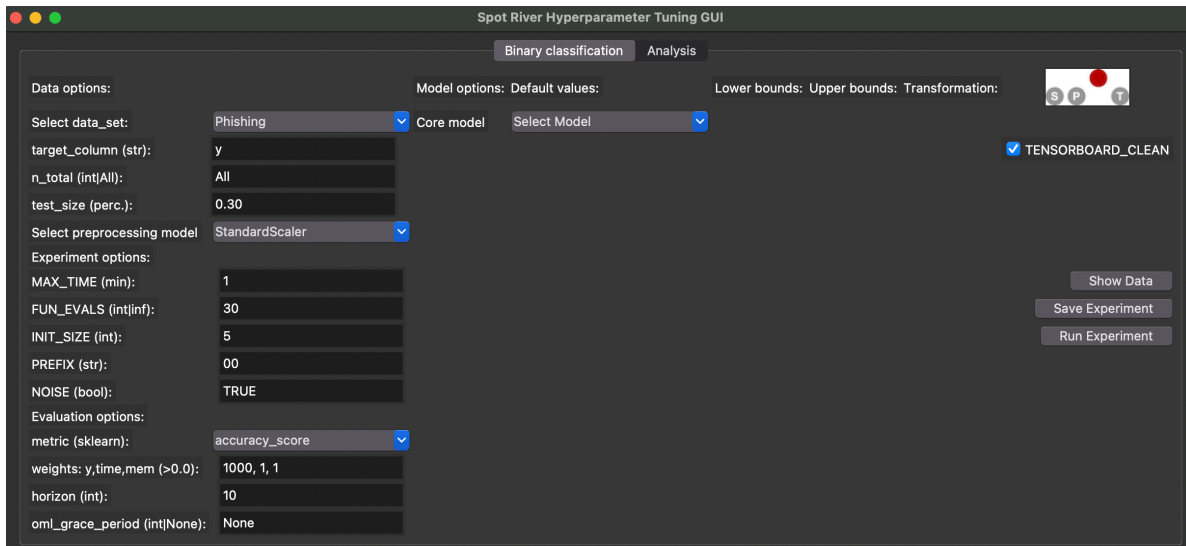
Figure 19.1: spotriver GUI
