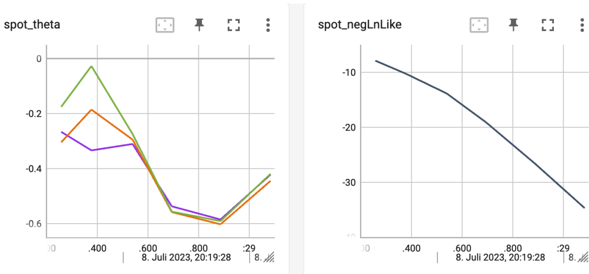
Figure 8.2: TensorBoard visualization of the spotPython surrogate model.
