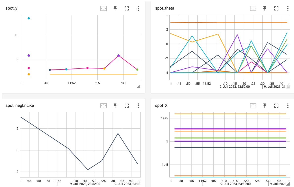
Figure 17.1: TensorBoard visualization of the spotPython optimization process and the surrogate model.
