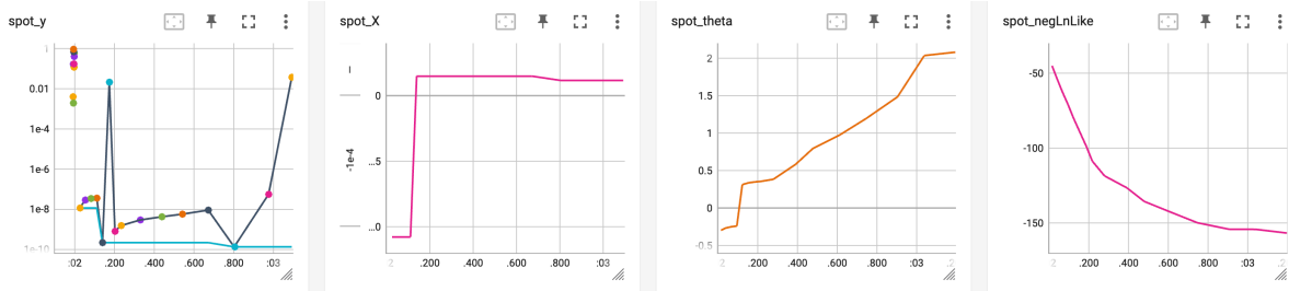
Figure 12.2: TensorBoard visualization of the spotPython optimization process and the surrogate model. Expected improvement, isotropic Kriging.
