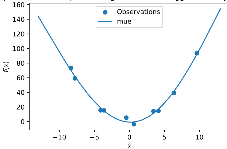
Sphere: Gaussian process regression with nugget on noisy dataset
