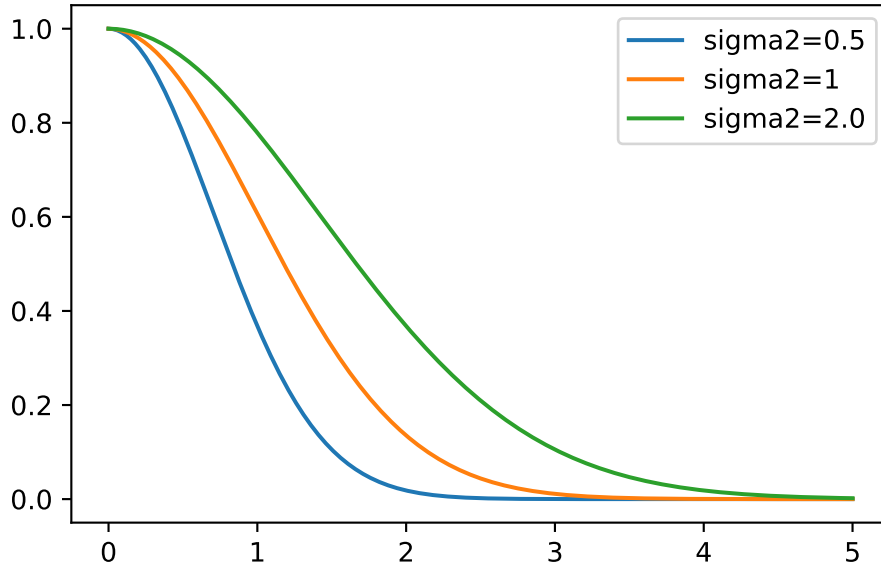
Figure 6.5: One-dim inverse exponentiated squared Euclidean distance
