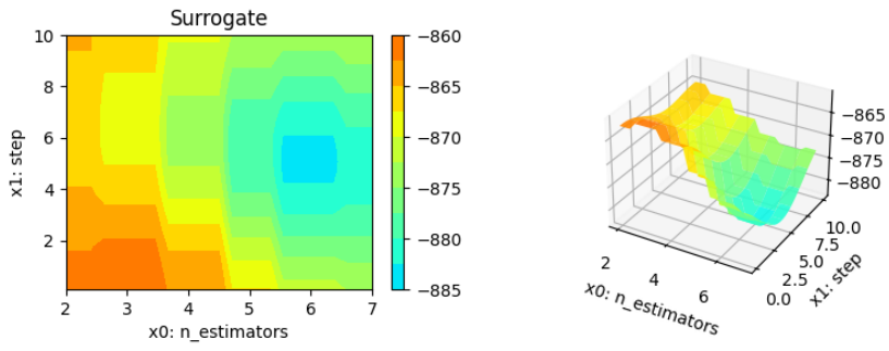
Figure 19.15: Surrogate plot based on the Kriging model. x_0 and x_1 plotted against each other.
