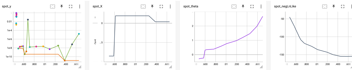
Figure 12.1: TensorBoard visualization of the spotPython optimization process and the surrogate model.
