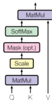
Figure 28.3: Scaled dot product attention. Figure credit Vaswani et al. (2017)
