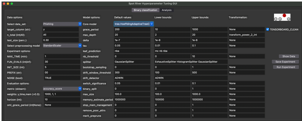
Figure 19.3: spotRiverGUI when tree.HoeffdingAdaptiveTreeClassifier is selected
