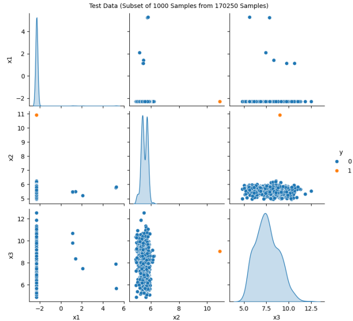
Figure 19.9: Output from the spotRiverGUI when HTTP data is selected for the Show Data option. The test data set shows the same structure as the train data set.
