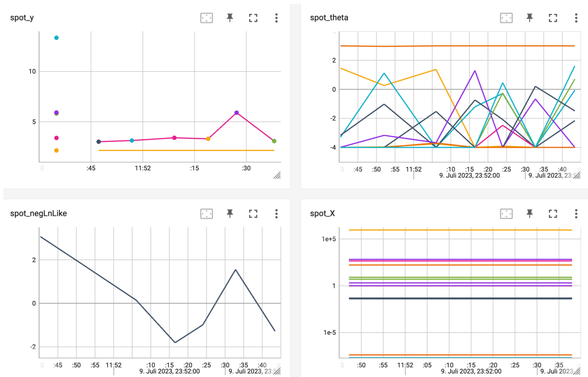
Figure 21.1: TensorBoard visualization of the spotPython optimization process and the surrogate model.
