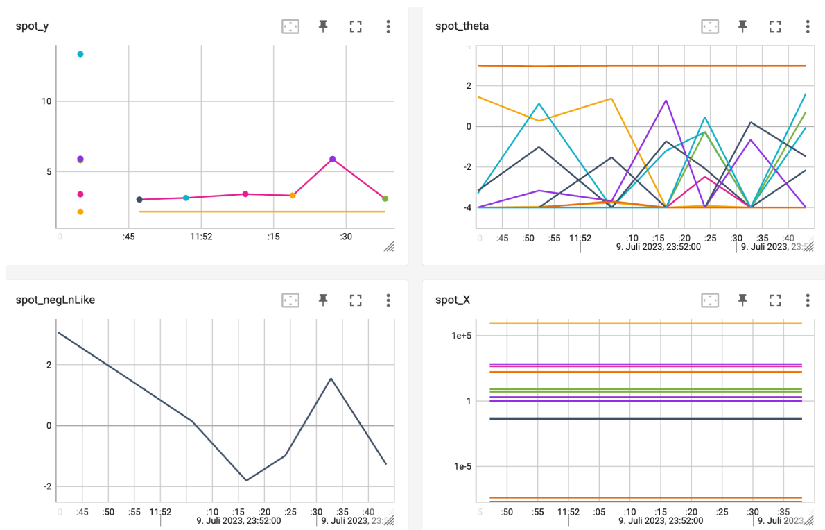
Figure 20.1: TensorBoard visualization of the spotPython optimization process and the surrogate model.
