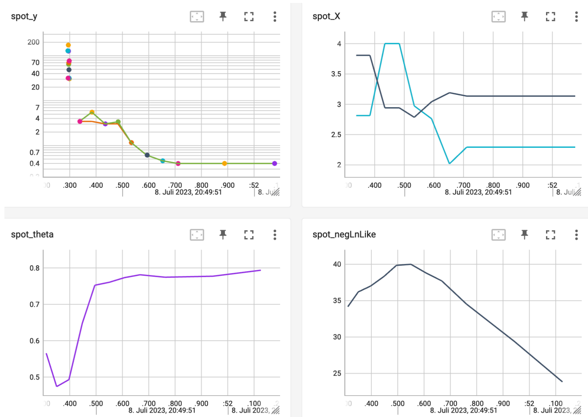
Figure 10.1: TensorBoard visualization of the spotPython optimization process and the surrogate model.
