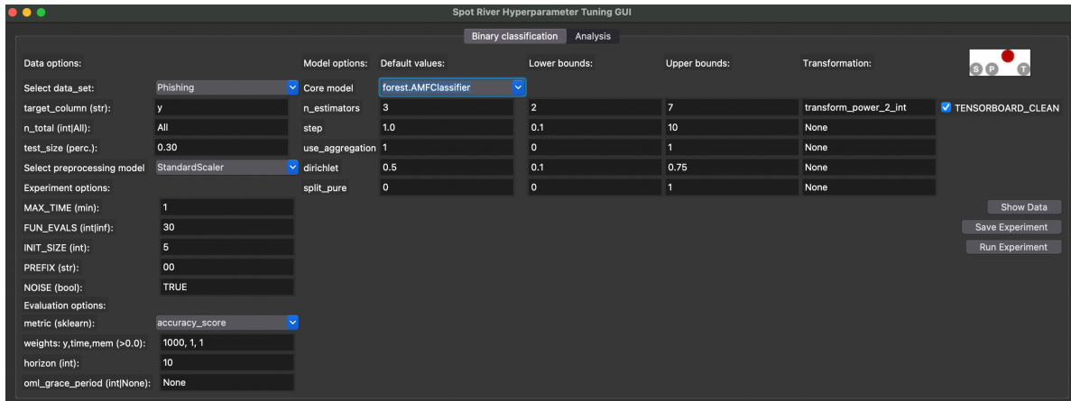
Figure 19.2: spotRiverGUI when forest.AMFClassifier is selected
