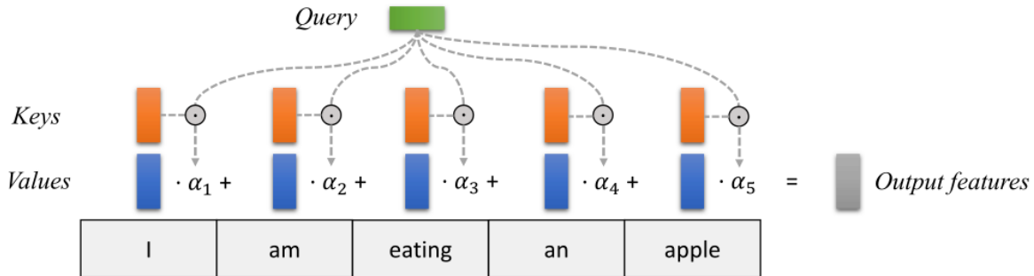
Figure 28.2: Attention over a sequence of words. For every word, we have one key and one value vector. The query is compared to all keys with a score function (in this case the dot product) to determine the weights. The softmax is not visualized for simplicity. Finally, the value vectors of all words are averaged using the attention weights. Figure taken from Lippe (2022)
