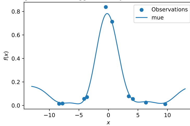
Gaussian process regression with nugget on noisy dataset. Modified Lambda search space.
