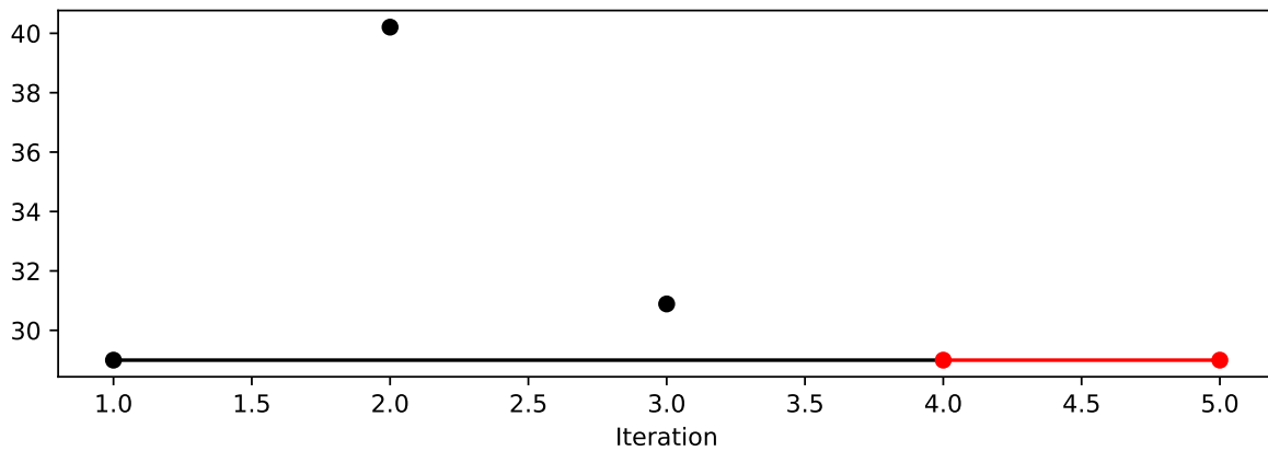
Figure 26.1: Progress plot. Black dots denote results from the initial design. Red dots illustrate the improvement found by the surrogate model based optimization.
