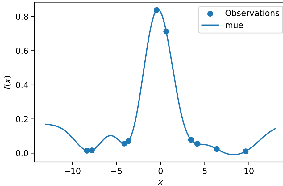
Gaussian process regression on noisy dataset
