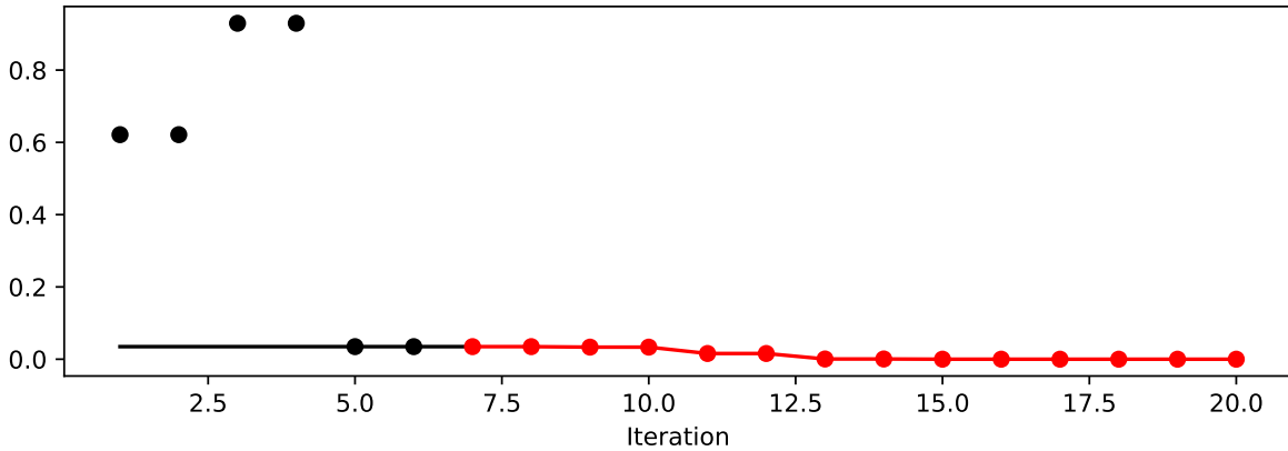
Figure 13.1: Progress plot. Black dots denote results from the initial design. Red dots illustrate the improvement found by the surrogate model based optimization.
