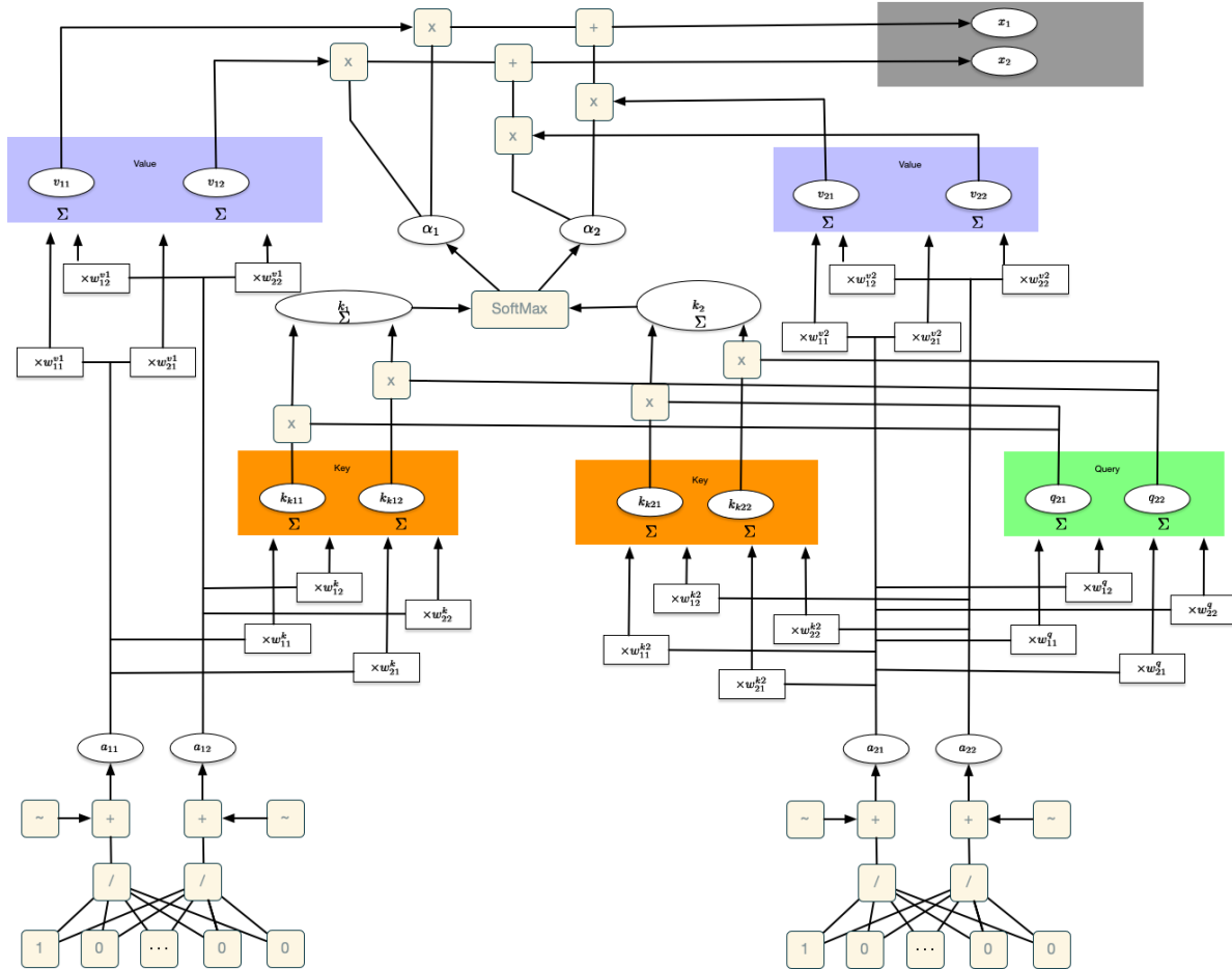
Figure 28.1: Transformer. Computation of the self attention. In this example, we consider two inputs, i.e., (1,0) and (0,1). For each input, there are two values, which results in a 2 \times 2 matrix. In general, when there are T inputs, a T \times T matrix will be generated. Figure credits: Starmer, Josh: Decoder-Only Transformers, ChatGPTs specific Transformer, Clearly Explained .
