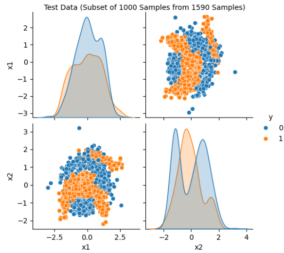
Figure 19.6: Visualization of the test data. Output from the spotRiverGUI when Bananas data is selected for the Show Data option
