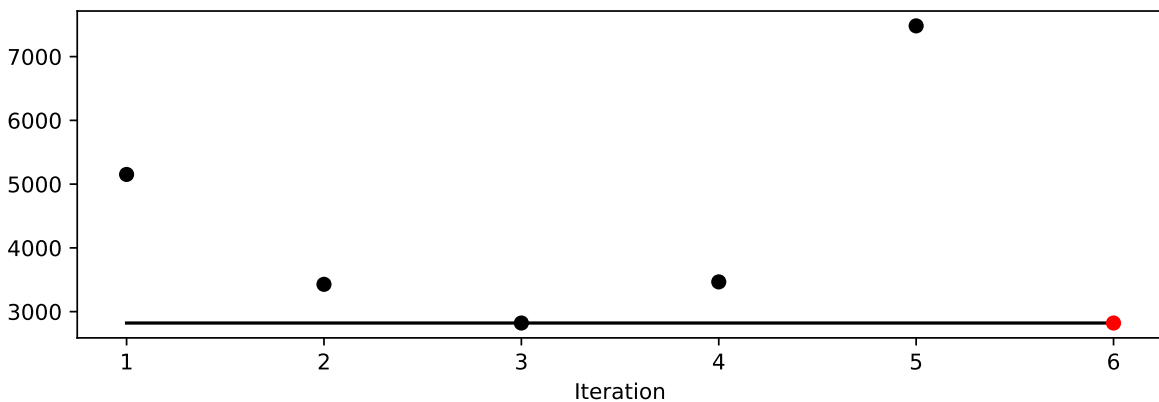
Figure 25.1: Progress plot. Black dots denote results from the initial design. Red dots illustrate the improvement found by the surrogate model based optimization.
