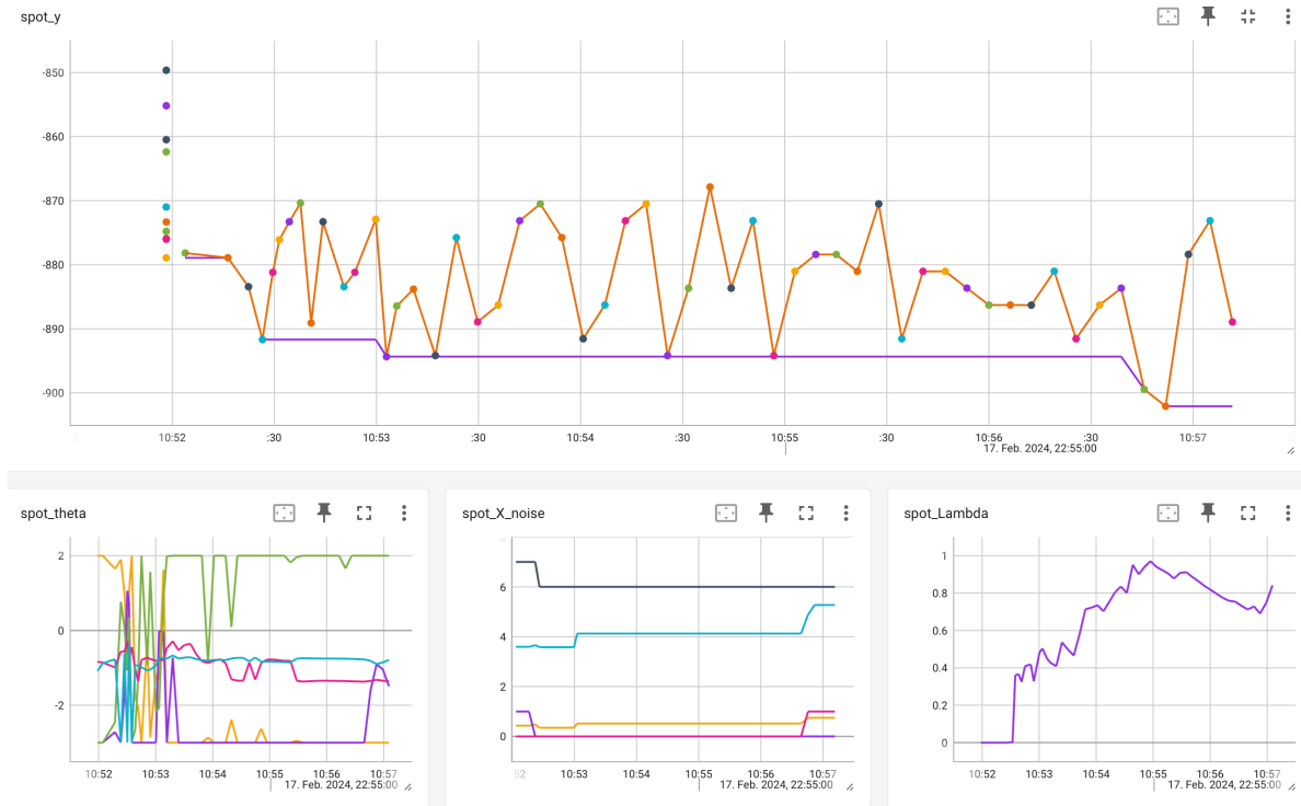
Figure 19.10: Tensorboard visualization of the hyperparameter tuning process
