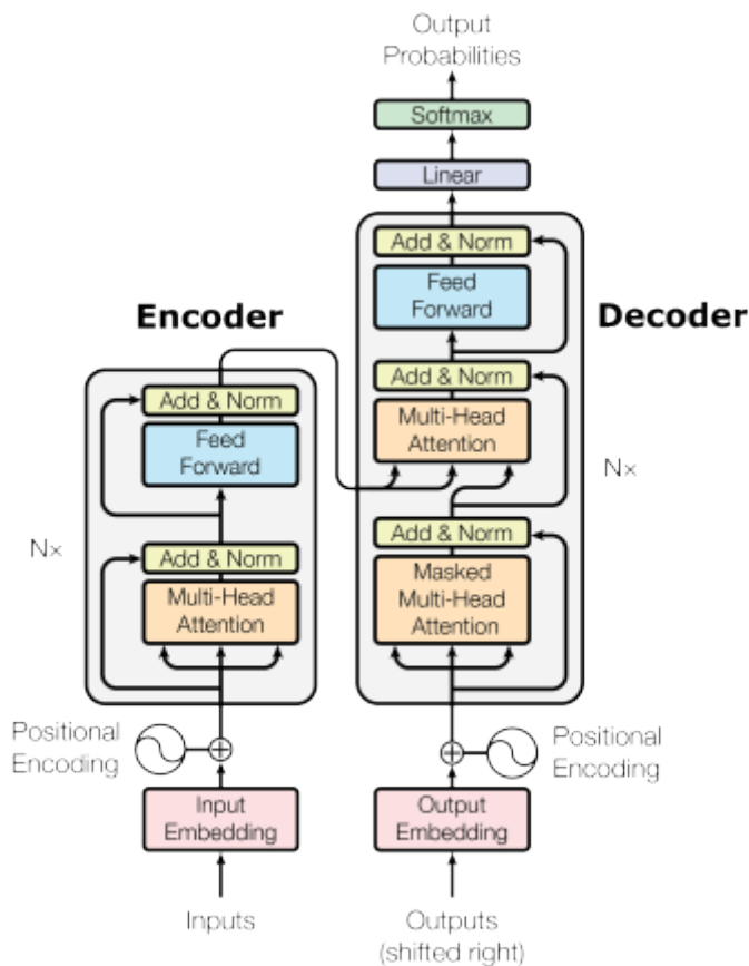
Figure 28.5: Transformer architecture. Figure credit: Vaswani et al. (2017)
