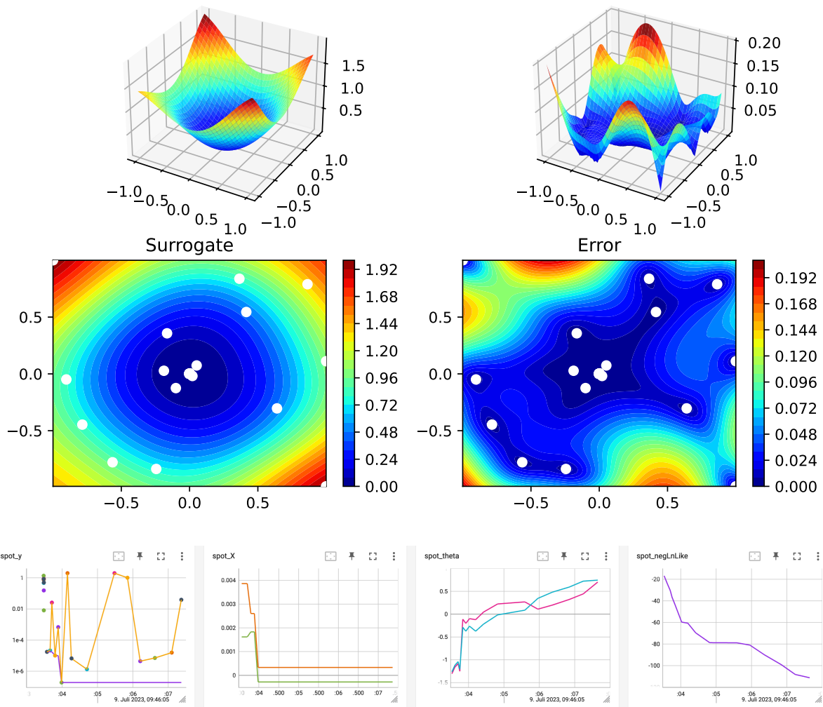
Figure 12.3: TensorBoard visualization of the spotPython optimization process and the surrogate model. Expected improvement, isotropic Kriging.
