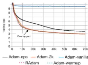
Figure 28.6: Warm-up comparison. Figure taken from Liu et al. (2019)
