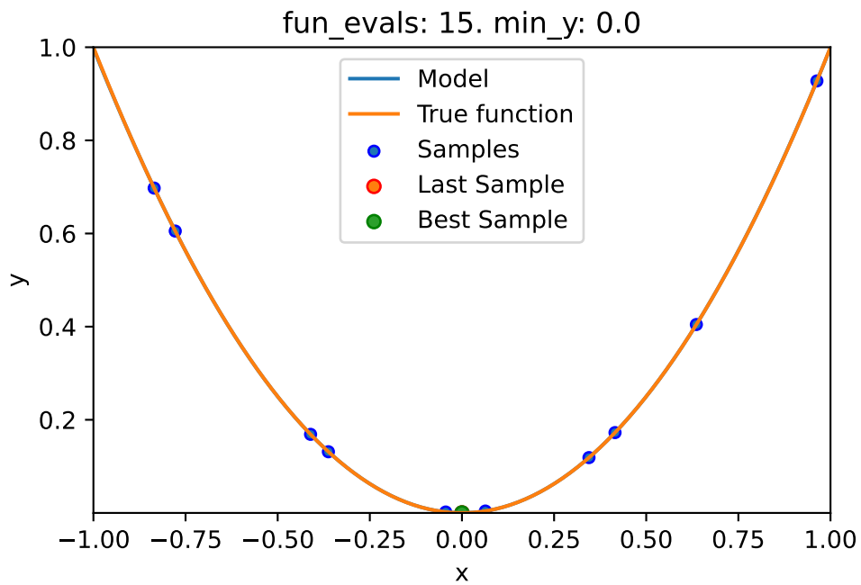
Figure 7.2: Visualization of the model and the underlying objective function values.
