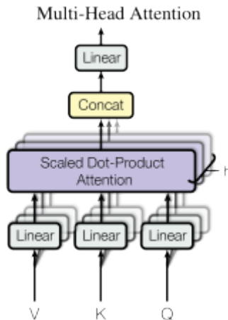
Figure 28.4: Multi-Head Attention. Figure taken from Vaswani et al. (2017)
